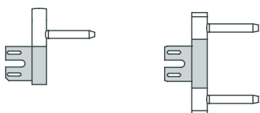
Hinge V 0020 Frame section V 8100 Hinge V 0026 WF Frame section V 8000
