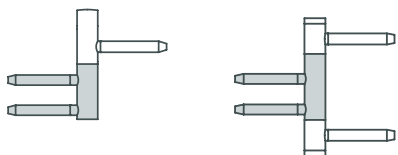
Hinge V 0020 Frame section V 3400 WF Hinge V 0026 WF Frame section V 4400 WF
