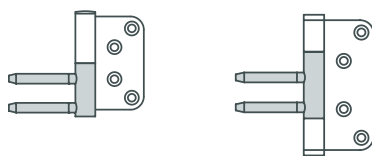
Hinge V 0080 Frame section V 3400 WF Hinge V 0087 WF Frame section V 4400 WF
