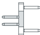
Hinge V 0026 WF Frame section V 4400 WF
